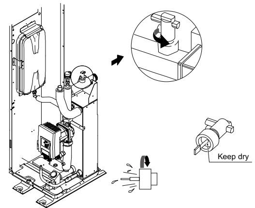
Figure 3-3.3: Air purge valve
