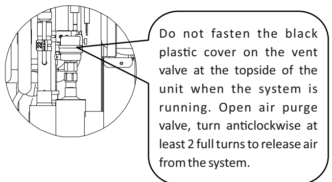
Figure 3-3.3: Air purge valve
