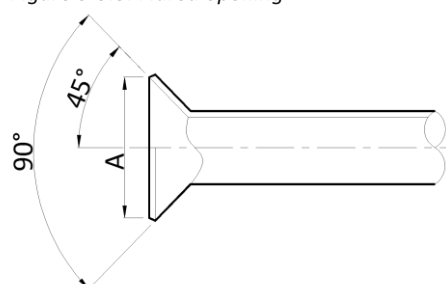
Figure 3-3.3: Flared opening
