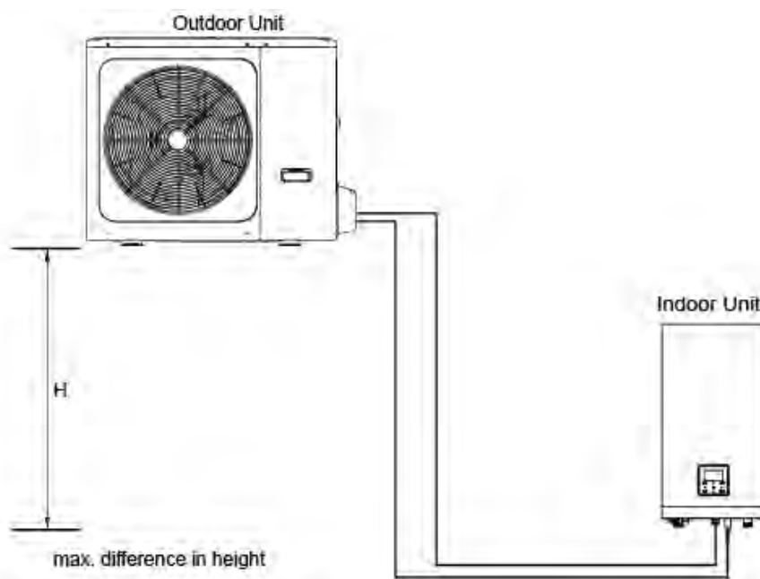
Figure 3-3.1: Connect method
