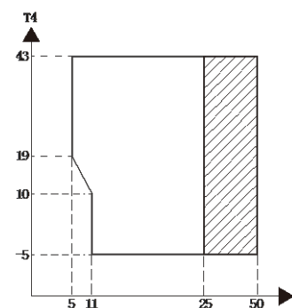
Figure 2-6.2: Cooling operating limits 1
