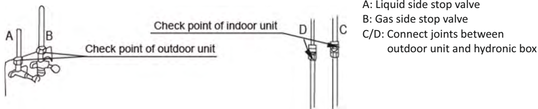
Figure 3-3.11: Leak detection
