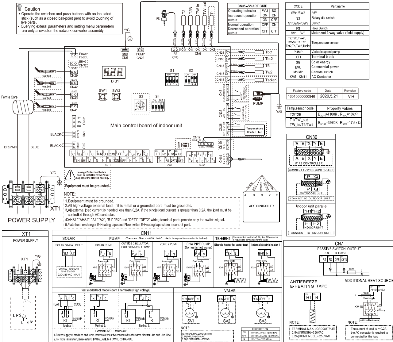
Figure 2-4.3: SHPAI60(100,160)RP24CM(-EH) wiring diagram
