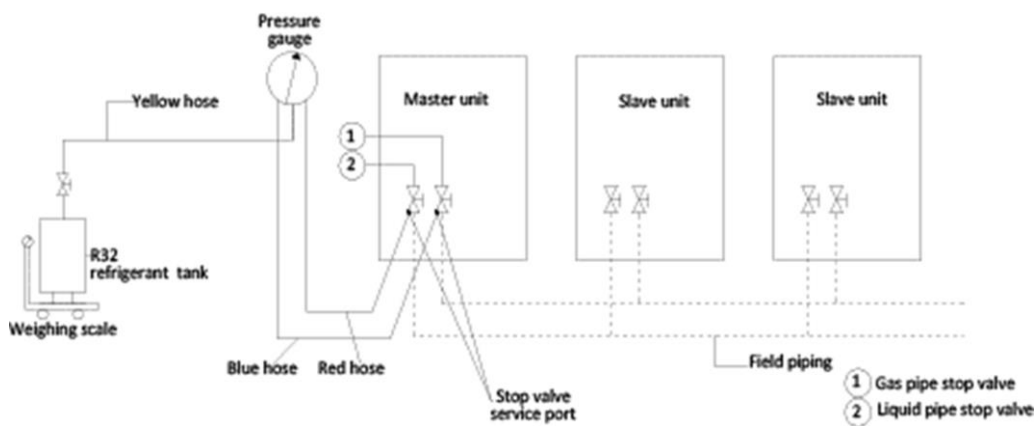
Figure 3-3.13: Charging refrigerant
