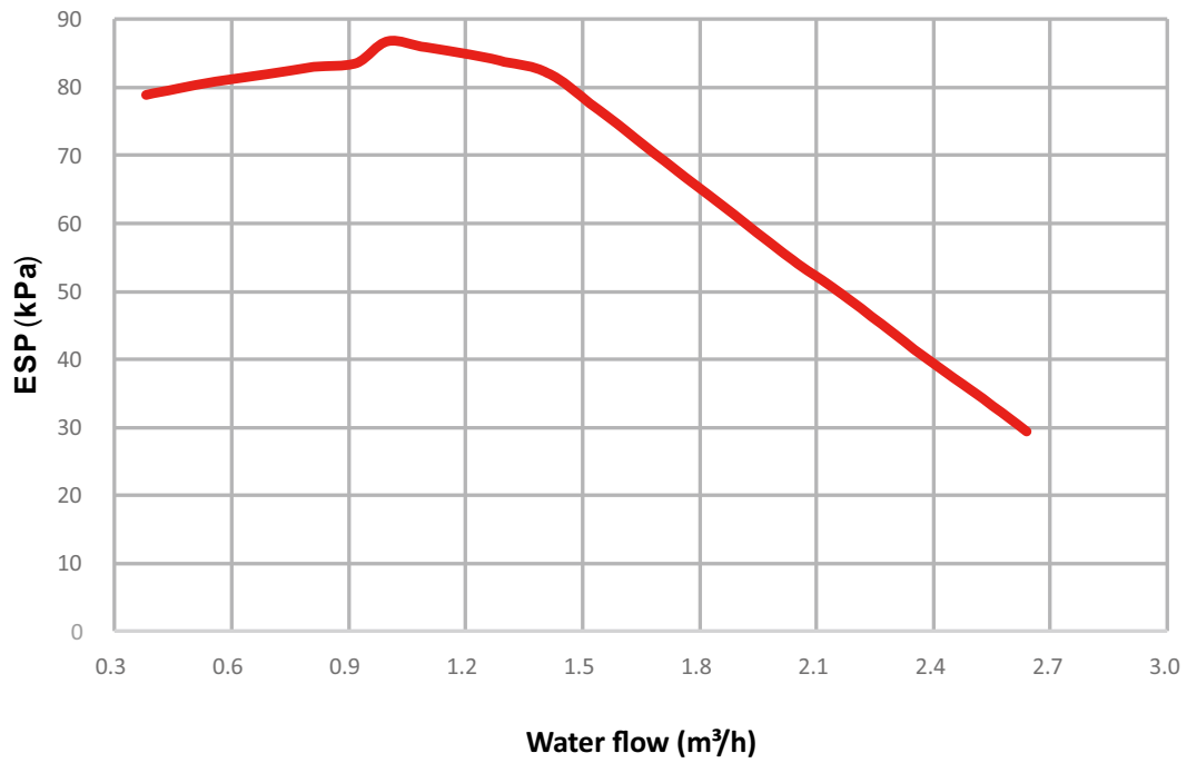
Figure 2-7.1: SHPAI60(100)RP24CM(-EH) hydronic performance
