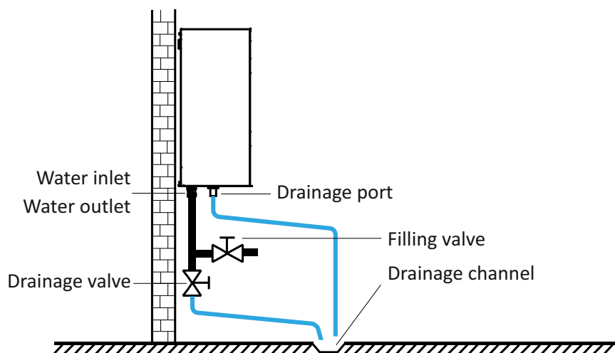
Figure 3-2.16: Drainage
