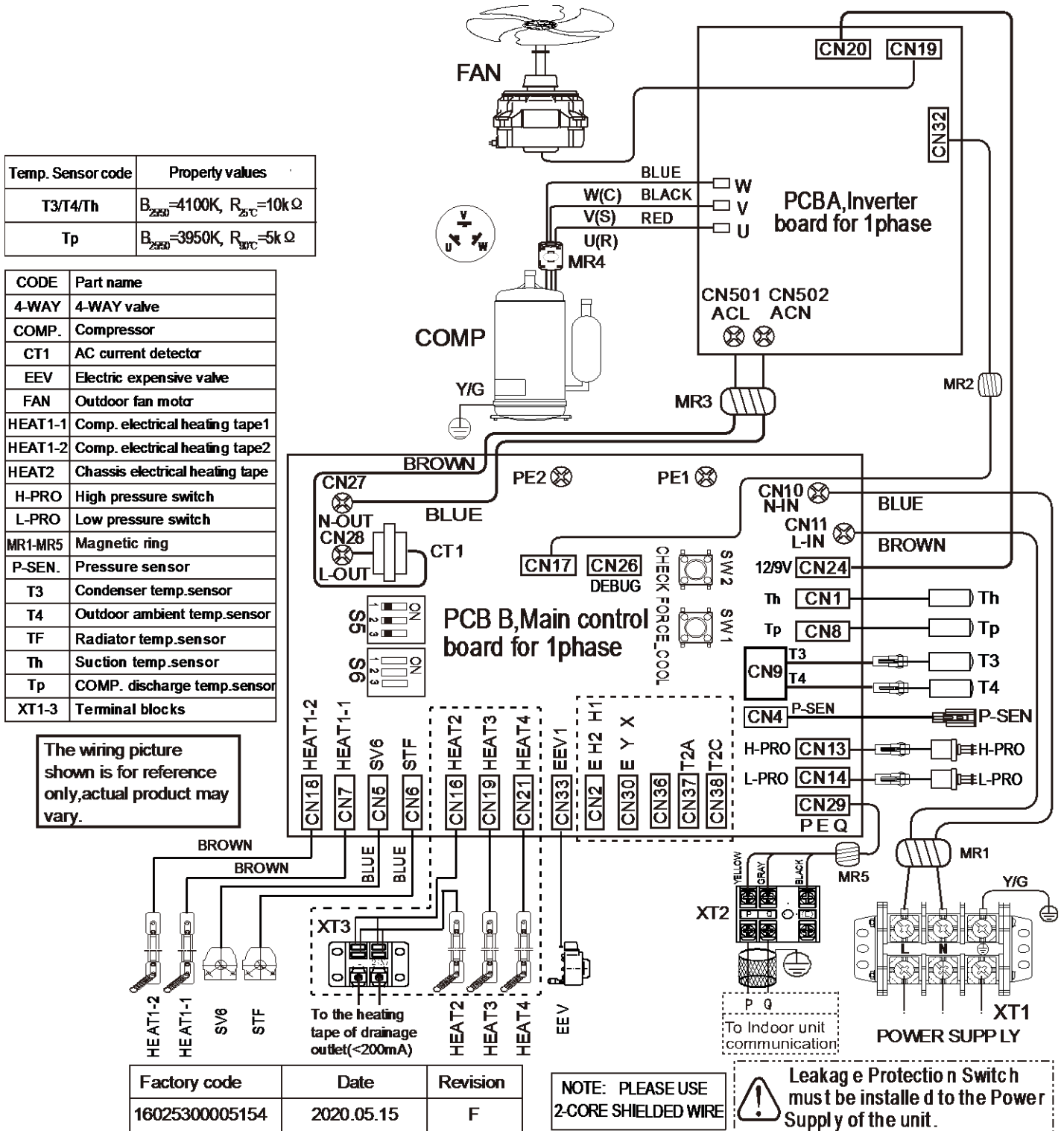
Figure 2-4.1: SHPA06(10)RP24CM wiring diagram
