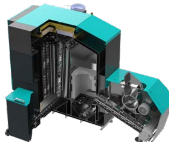
Boiler cross section
