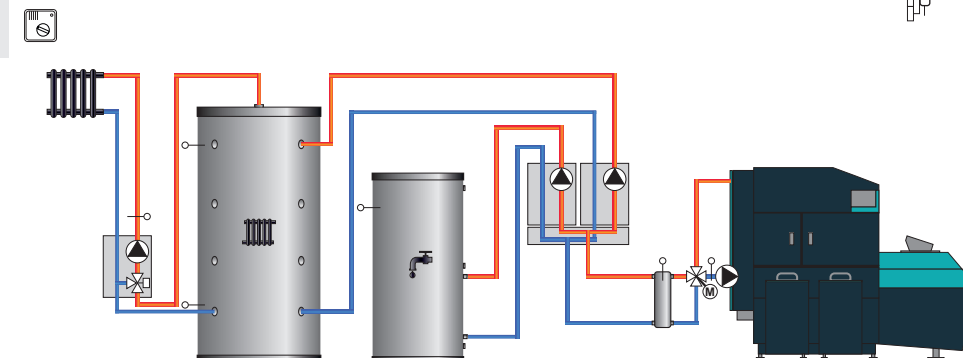
One of the possible 45 schemes of connection to the heating system and DHW with basic equipment
