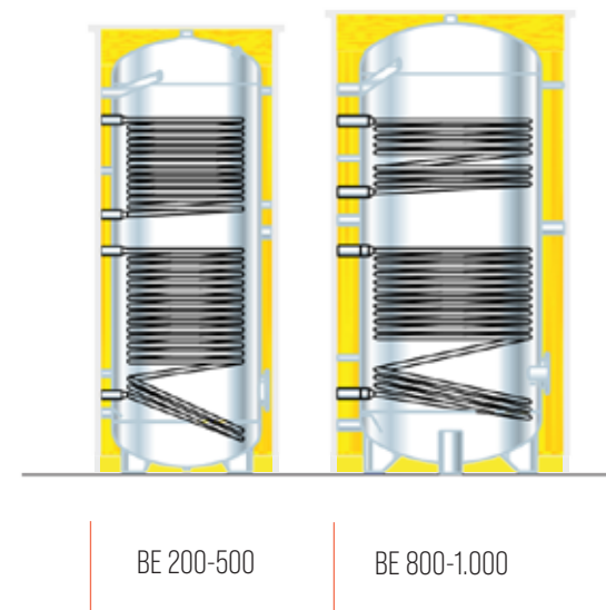
BE cross section
