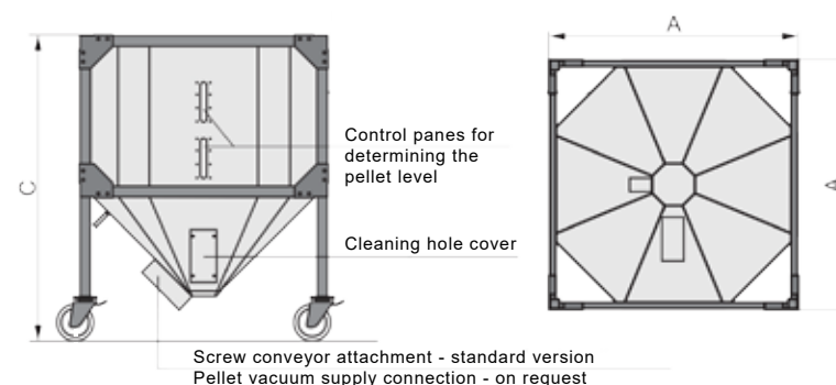
CentroPelet box 1500-4000
