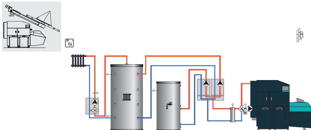
One of the possible 45 schemes of connection to the heating system and DHW with basic equipment
