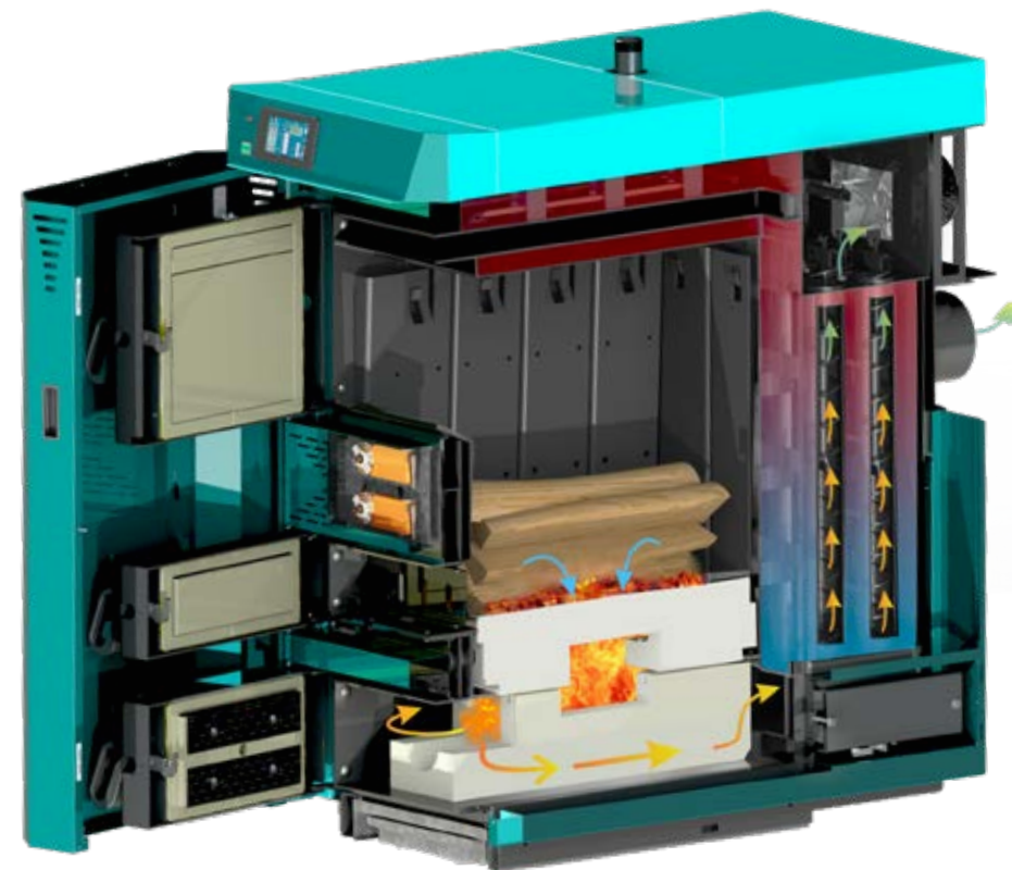
Boiler cross section
