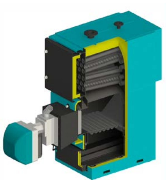
Boiler cross section
